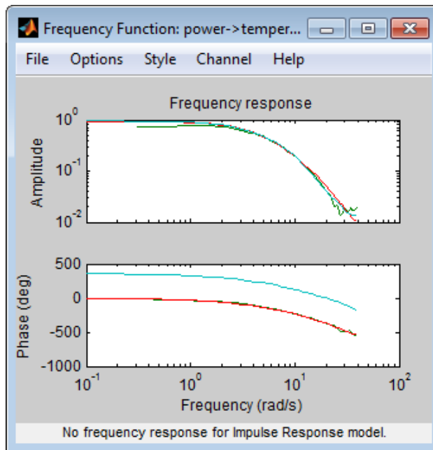
Frequency Response for Models spad, arxqs, and n4s3
