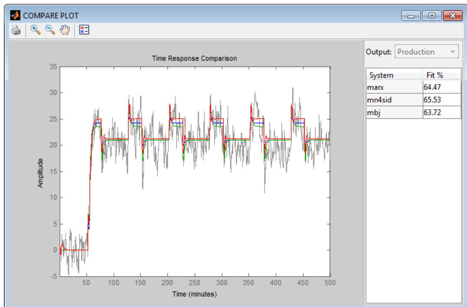
Measured Output and Simulated Outputs
